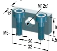
MB12SC2 Montageblock
