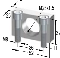
MB25SC2-V4A Montageblock
