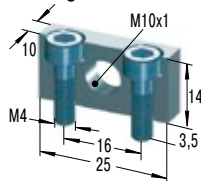
MB10SC2 Montageblock
