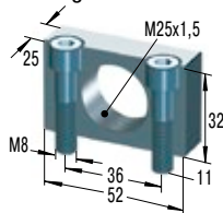
MB25SC2 Montageblock
