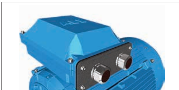
Fig. 5. Terminal box for motor sizes 280 – 315 SM-ML. Adapter and cable sealing end unit.
