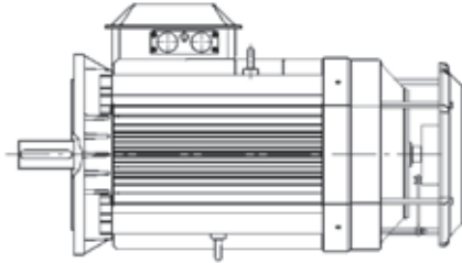
Tachometer, variant codes 472, 473, 572, and 573
