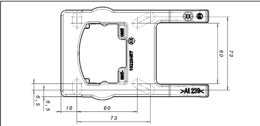
Abb. 21: Bohrbild Standard-Adapterplatte BG A
