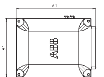
Motor sizes 355 to 400. side-mounted. terminal box 750
