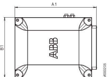
Motor sizes 280 to 315
