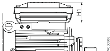
Motor sizes 80 to 132
