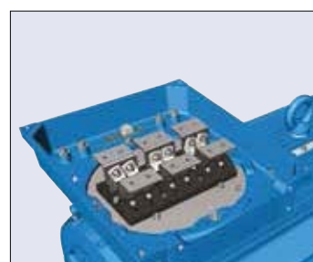
Fig 12. Terminal board for motor size 450.
