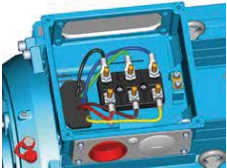
Terminal box size 200-280
