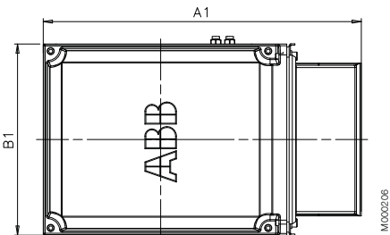
Motor sizes 355 to 400
